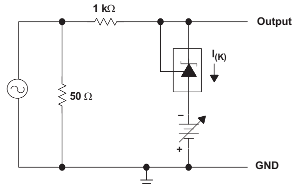
Figure 18. Test Circuit For Reference Impedance
